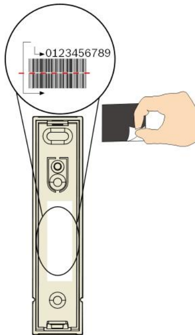
Figure 3.3: RFID sticker example (RFDW-SM-A shown)
